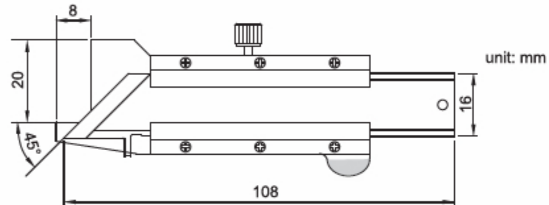
measure 45° chamfer dimension
