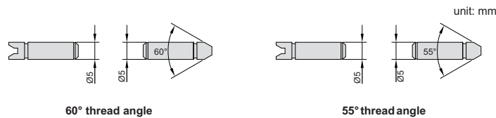
60° thread angle
