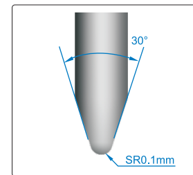
HSM5D indenter
